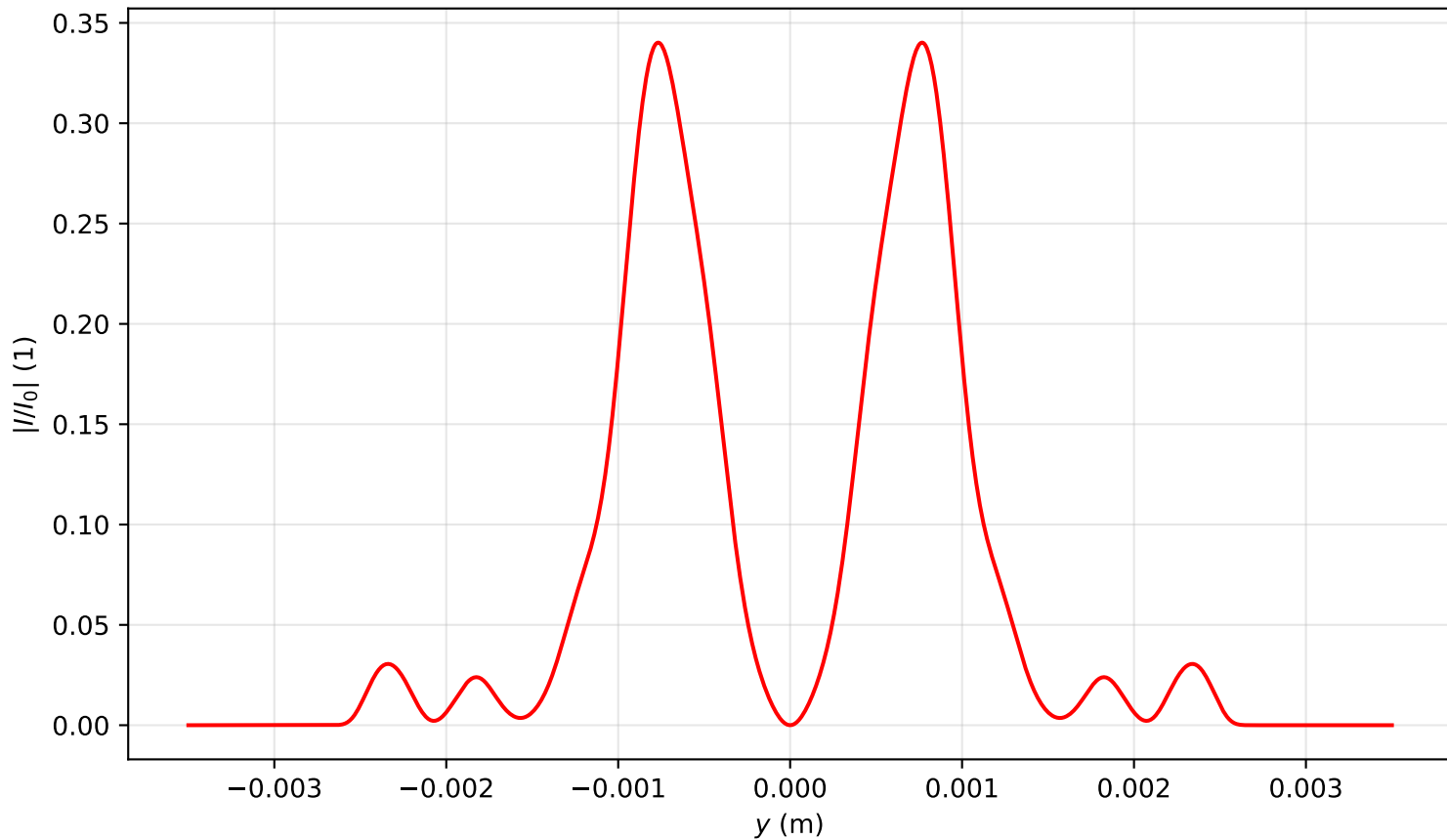
Intensity profile I(x=0, y, z=3.264)/I_0 , P_{in}=6.0P_{cr} , artificial time
